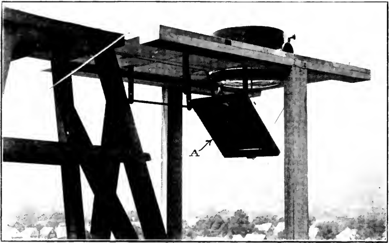
When used as a Landing Light on an Airplane, the Convex-Mirror A was lowered as shown and the beam directed to any spot on the Landing Field
